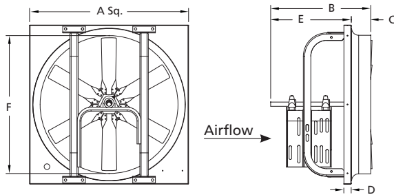
Figure 1 — Exhaust Dimensions
