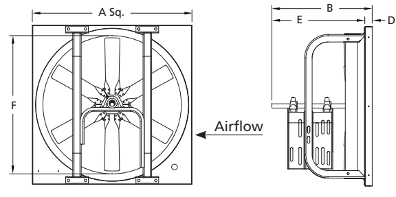
Figure 2 — Supply Dimensions
